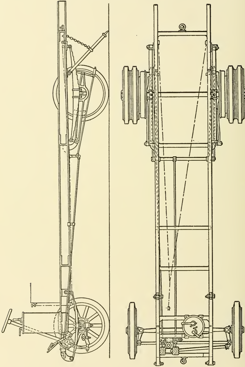
Fig. 10. Plan and Elevation of Mercedes Chassis. The Motors Are Mounted Inside the Double-Tired Rear Wheels
